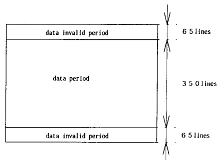
350 lines mode (TV=449)
